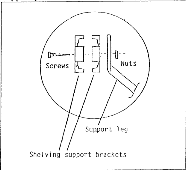
Support post used when two shelves meet
