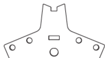
BXU (x2) Truss Connector A
