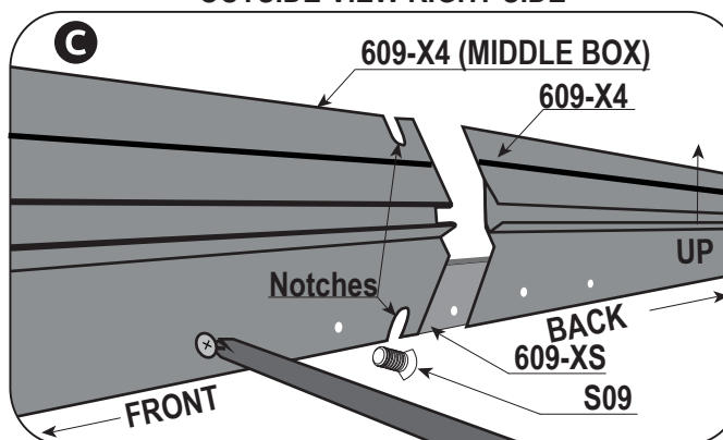
OUTSIDE VIEW RIGHT SIDE
