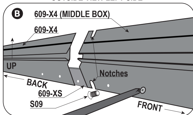
OUTSIDE VIEW LEFT SIDE
